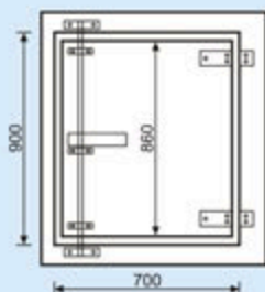
Porta laterale supplementare obbligatoria per kit IR Side supplementary door is obligatory for IR kit - Porte latérale supplémentaire obligatoire pour IR kit Puerta lateral suplementaria obligatoria para el kit
