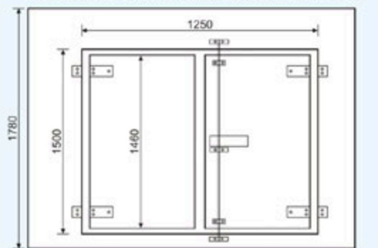
PORTA LATERALE SUPPLEMENTARE - SUPPLEMENTARY SIDE DOOR PORTE LATÉRALE SUPPLÉMENTAIRE - PUERTA LATERAL SUPPLEMENTARIA
