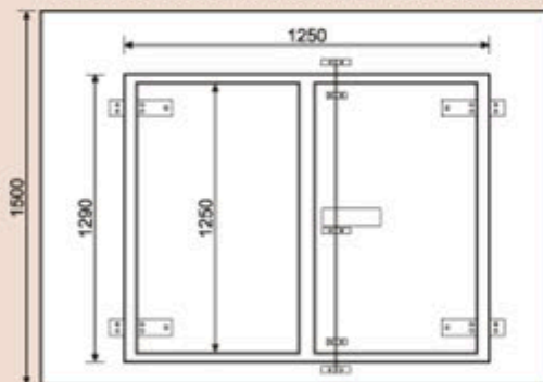
PORTA LATERALE SUPPLEMENTARE - SUPPLEMENTARY SIDE DOOR PORTE LATÉRALE SUPPLÉMENTAIRE - PUERTA LATERAL SUPLEMENTARIA
