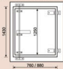
Porta laterale supplementare obbligatoria per kit IR Side supplementary door is obligatory for IR kit - Porte latérale supplémentaire obligatoire pour kit IR Puerta lateral suplementaria obligatoria para el kit
